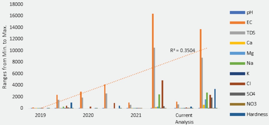
Figure 14. Comparison of the analysis of Hydrogeochemical parameters with published data - 2019 to 2021 [29, 39-40]
