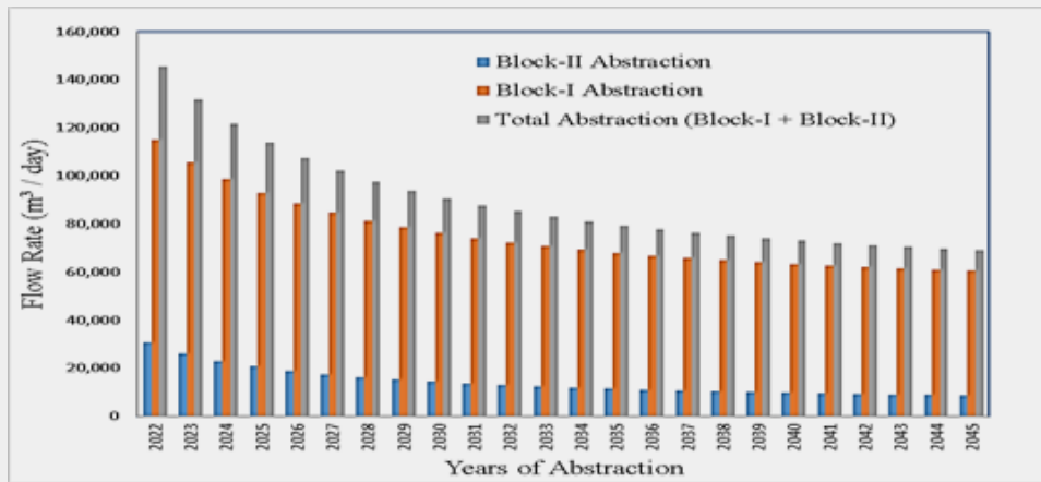
Figure 25. Predicted rate of abstractions for Block-I and Block-II under low flow condition ( K = 7.5 m/ day)
