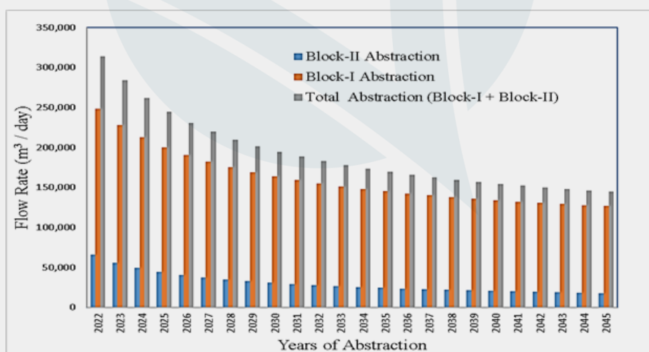
Figure 24. Predicted rate of abstractions for Block-I and Block-II under high flow condition ( K = 16.4 m/ day)
