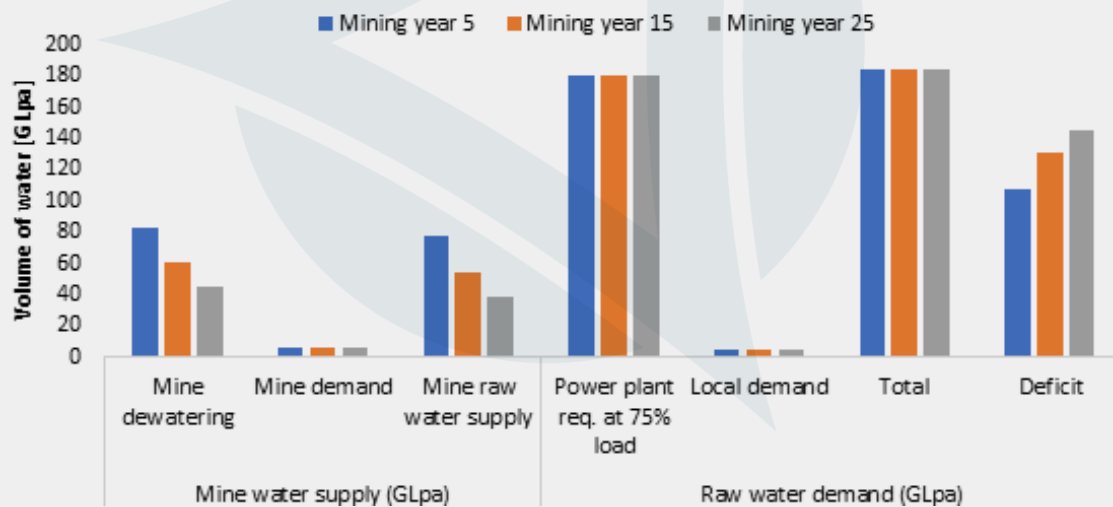
Figure 16. Water Balance for Thar coalfields
