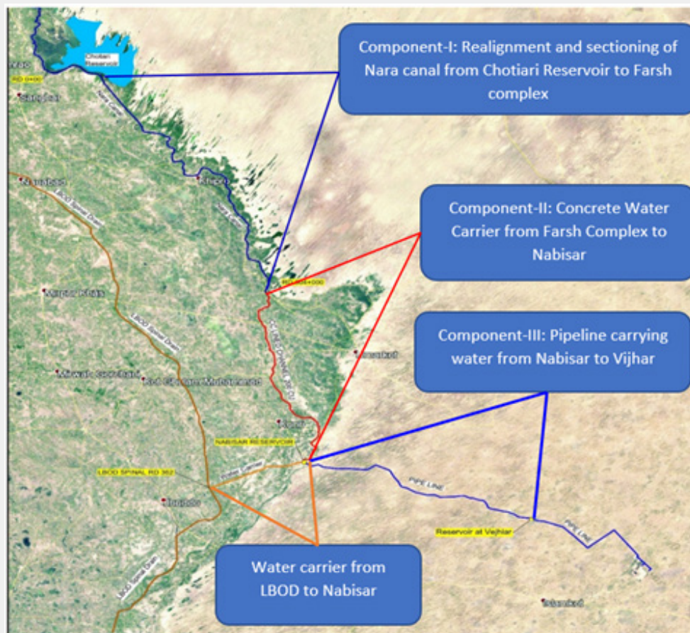
Figure 18. The map of the entire system carrying water from Nara Canal and LBOD to Nabisar water ponds and from Nabisar to Vijhar water ponds [47]
